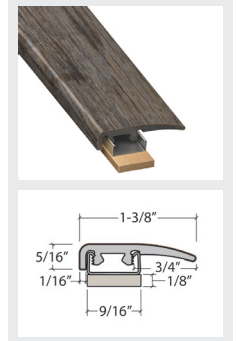
SlimCap with Track and Shim
